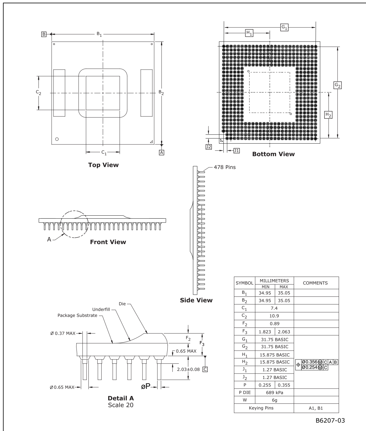
Figure 6. 1-MB Micro-FCPGA Processor Package Drawing (1 of 2)
