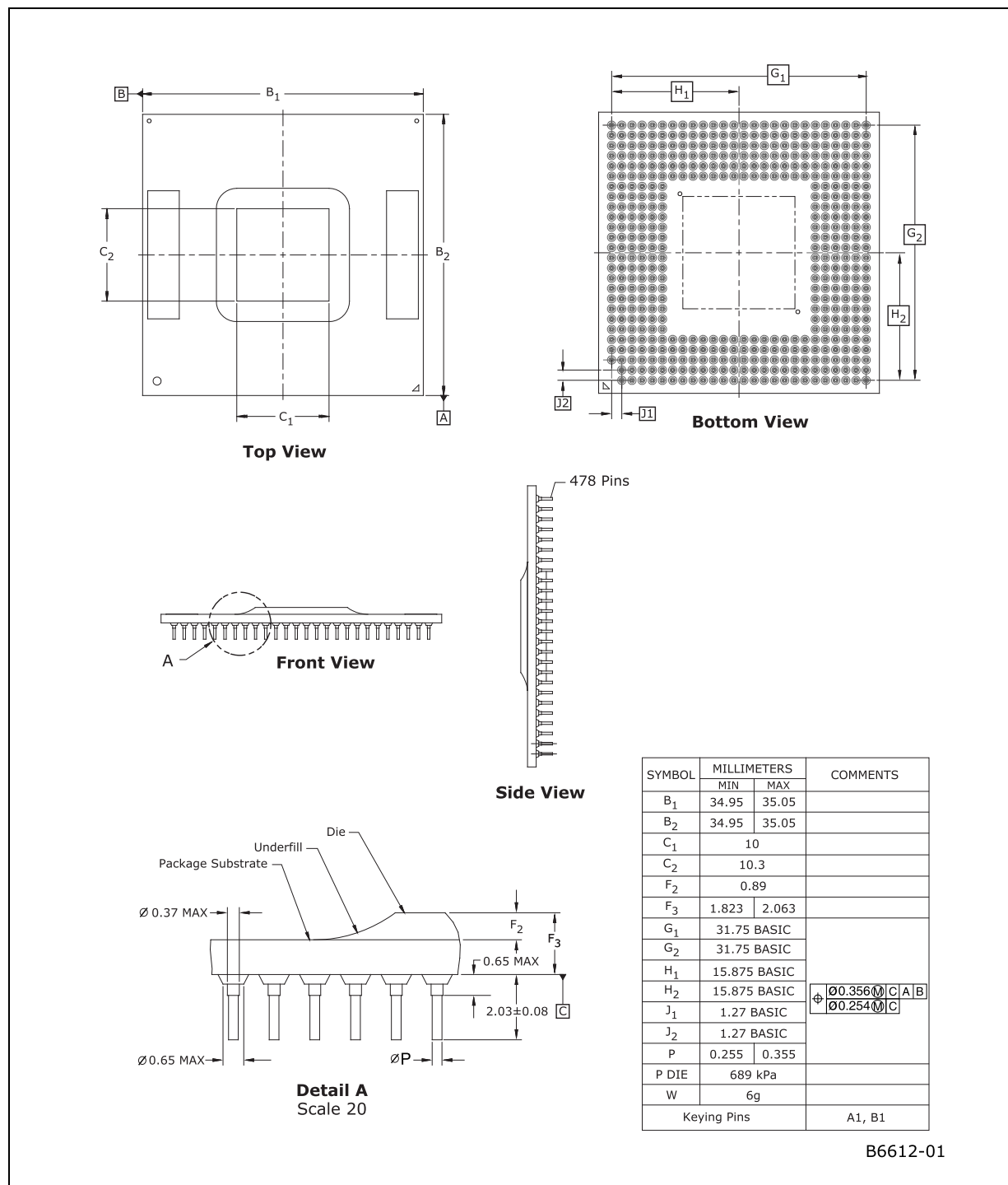
Figure 4. 1-MB Fused Micro-FCPGA Processor Package Drawing (1 of 2)
