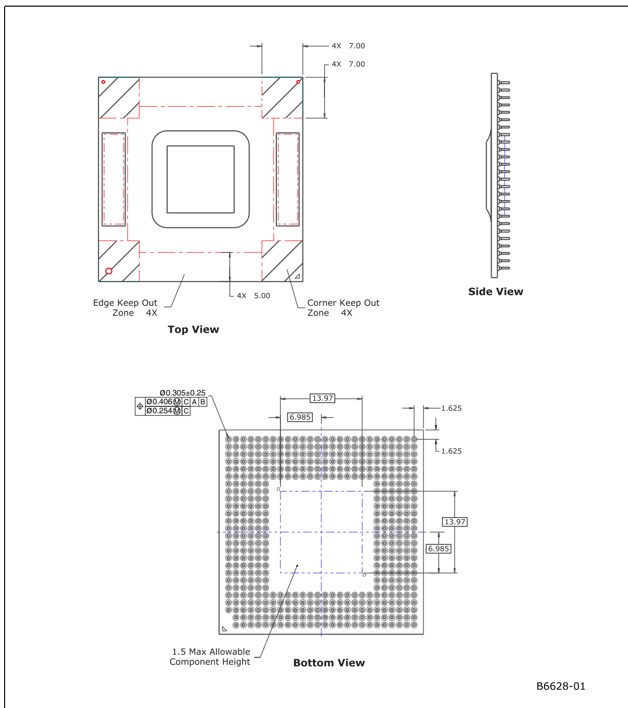
Figure 5. 1-MB Fused Micro-FCPGA Processor Package Drawing (2 of 2)
