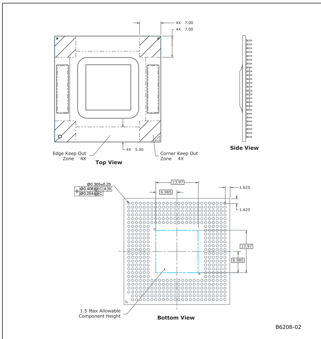
Figure 7. 1-MB Micro-FCPGA Processor Package Drawing (2 of 2)
